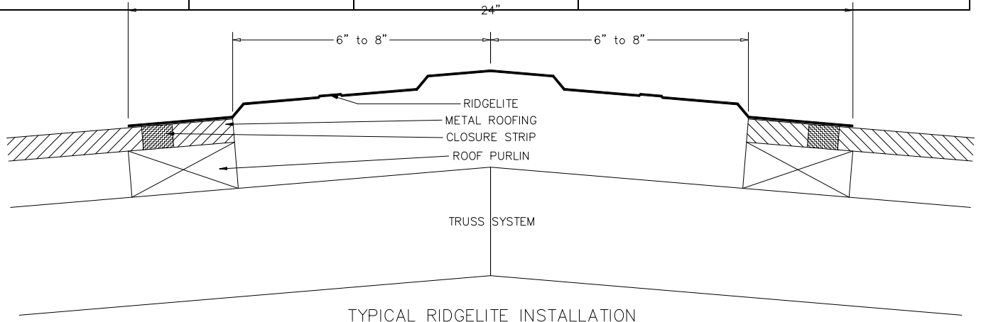
TYPICAL RIDGELITE INSTALLATION
