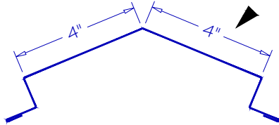
RIDGE CAP RC-04
