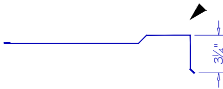
PROW GABLE GB-P2
