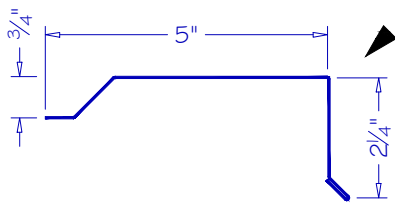
GABLE GB-01
