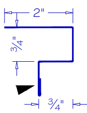
3/4" DOUBLE J ISC-07
