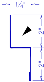
GABLE DIVIDER GD-03
