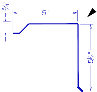
GABLE GB-03
