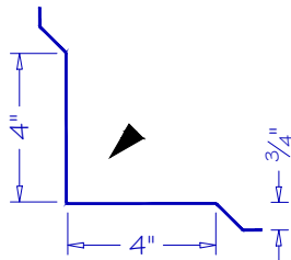
INSIDE CORNER ISC-02
