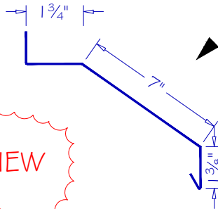
FACE MOUNT TC-03
