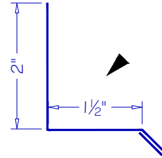
BASE BF-02
