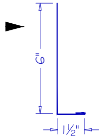
FASCIA FC-02
