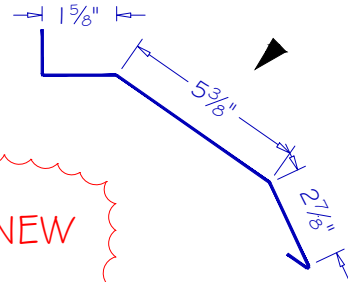
BIG FRAME FACE MOUNT TC-02
