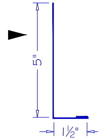
FASCIA FC-01
