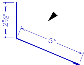
END WALL EW-01
