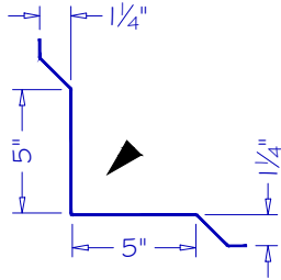
INSIDE CORNER ISC-05
