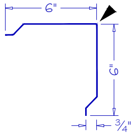
OUTSIDE CORNER OSC-03
