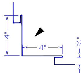
INSIDE CORNER ISC-03
