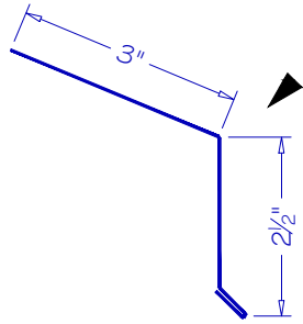
EAVE EV-02
