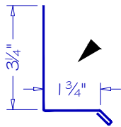
BASE BF-03
