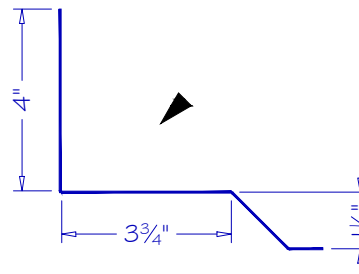
SIDE WALL SW-02
