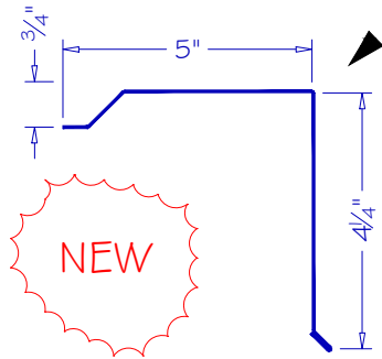
GABLE GB-05
