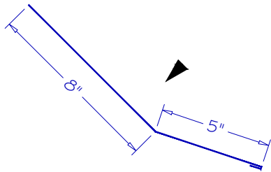
PITCH TRANSITION PT-02
