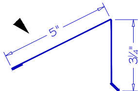
PEAK CAP PC-02
