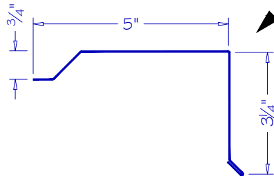
GABLE GB-02
