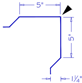
OUTSIDE CORNER OSC-05
