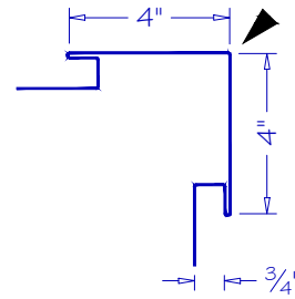
OUTSIDE CORNER OSC-04
