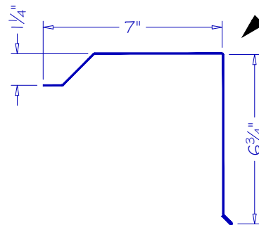
GABLE GB-04
