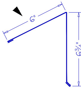
PEAK CAP PC-04
