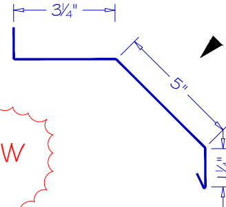
TOP MOUNT TC-04
